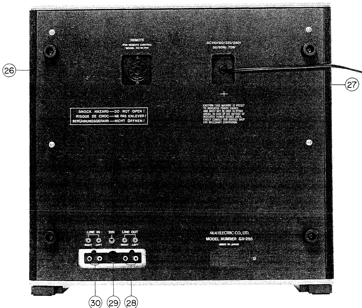
Fig. 1 Controls
