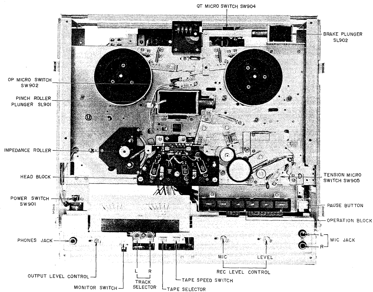
Fig. 2 Front View
