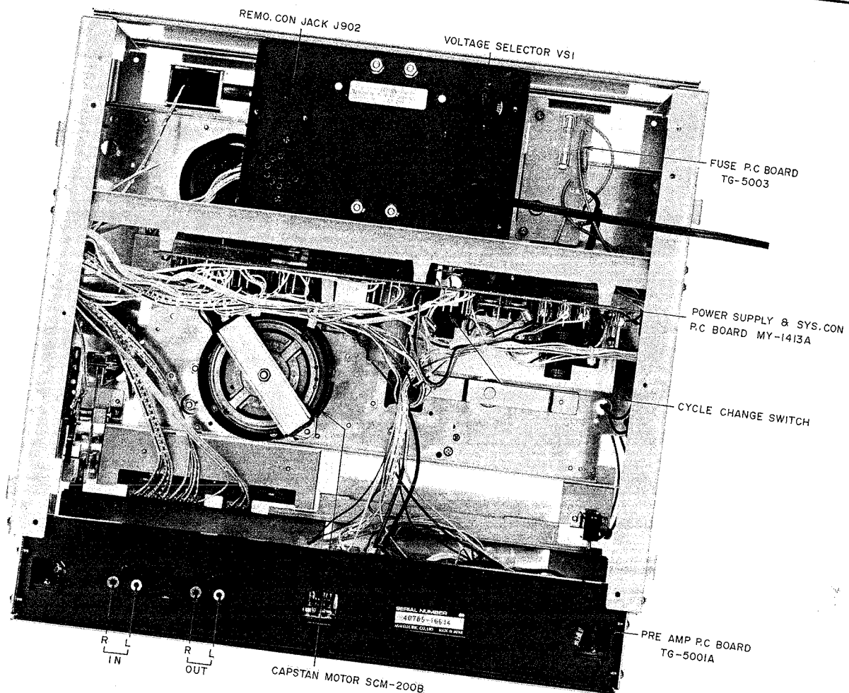
Fig. 3 Rear View
