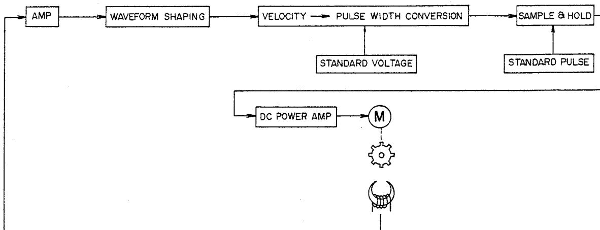
Fig. 7 Block Diagram
