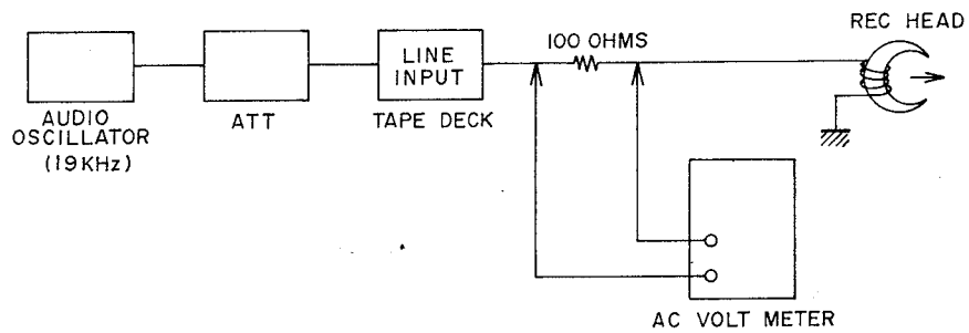
Fig. 24 Rec Peaking Adjustment Instrument Connection
